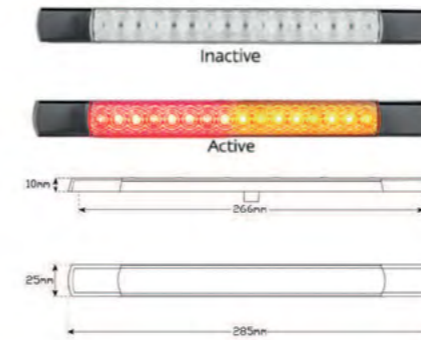
LED Autolamp 12V Stop/Tail/Indicator Taillight
