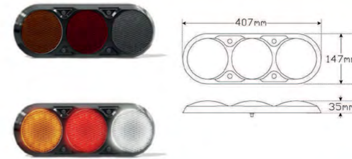
LED Autolamp Triple Surface Tail lamp Mount Housing
