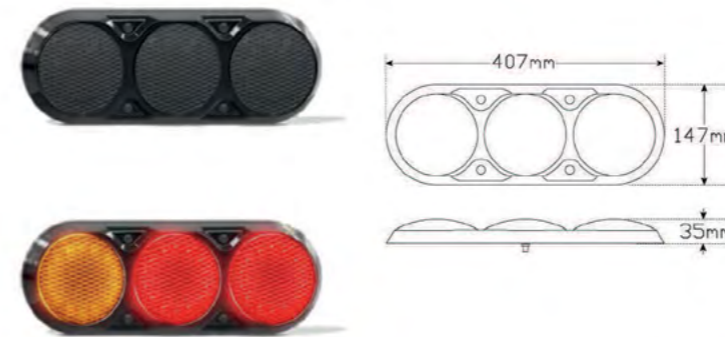
LED Autolamp 12V Slim Line Stop/Tail/Indicator Tail light
