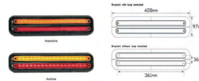
CCA-380BAR12: Black 428x97x22mm
