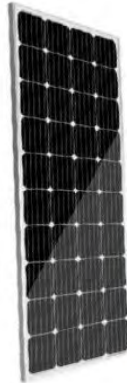
190W SOLAR PANEL 1480 x 670 x 30mm - BLACK ILU-SP190
